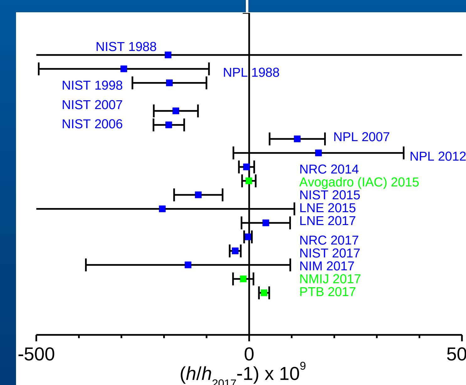
Comparison Measurements to Enable Redefinition of the Kilogram
